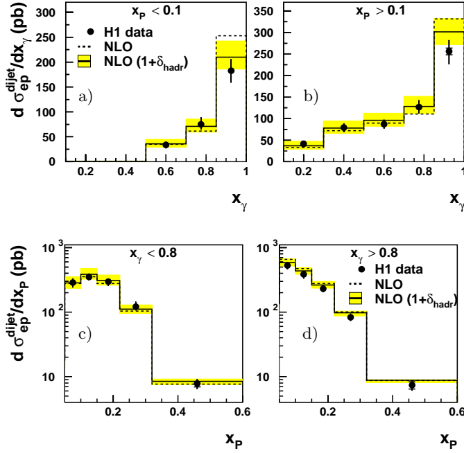
Fig. 4a–d. Differential ep cross sections for dijet production ( Q^2 < 1\text{GeV}^2 ) as a function of x_\gamma a and b and x_p c and d . a and b distinguish regions of small and large x_p and c and d corresponding regions in x_\gamma . NLO predictions using CTEQ5M pdfs for the proton and GRV-HO pdfs for the photon are shown as a dashed line . The full line shows the NLO predictions, including hadronization corrections and the grey band indicates the renormalization and factorization scale uncertainties of the NLO prediction
