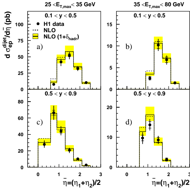
Fig. 3a–d. Differential ep cross sections for dijet production ( Q^2 < 1\text{GeV}^2 ) as a function of the \bar{\eta} of the two highest E_T jets. The regions of low y , a and b and high y , c and d are shown for two ranges of E_{T,max} . NLO predictions using CTEQ5M pdfs for the proton and GRV-HO pdfs for the photon are shown as a dashed line . The full line shows the NLO predictions, including hadronization corrections and the grey band indicates the renormalization and factorization scale uncertainties of the NLO prediction
