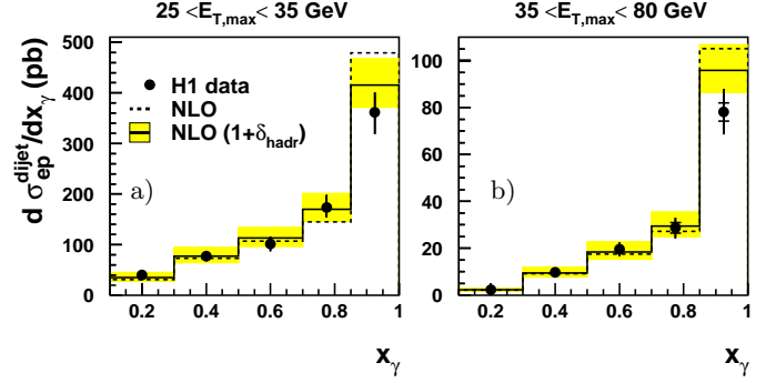
Fig. 6a,b. Differential ep cross sections for dijet production ( Q^2 < 1\text{GeV}^2 ) as a function of x_\gamma for a low E_{T,max} and b high E_{T,max} . NLO predictions using CTEQ5M pdfs for the proton and GRV-HO pdfs for the photon are shown as a dashed line . The full line shows the NLO predictions, including hadronization corrections and the grey band indicates the renormalization and factorization scale uncertainties of the NLO prediction
