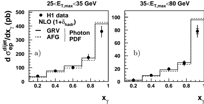
Fig. 5a,b. Differential ep cross sections for dijet production ( Q^2 < 1\text{GeV}^2 ) as a function of x_\gamma for a low E_{T,max} and b high E_{T,max} . The NLO predictions using CTEQ5M pdfs for the proton and GRV-HO pdfs for the photon and including hadronization corrections are shown as a full line. NLO predictions using AFG-HO parametrizations of the photon pdfs and including hadronization corrections are shown as the dashed line
