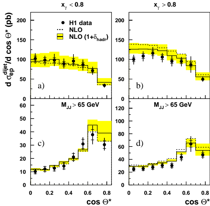
Fig. 8a–d. Differential ep cross sections for dijet production ( Q^2 < 1\text{GeV}^2 ) as a function of \cos\theta^* distinguished for small x_\gamma a and c and large x_\gamma b and d . c and d show the cross sections for large invariant masses of the dijet system. NLO predictions using CTEQ5M pdfs for the proton and GRV-HO pdfs for the photon are shown as a dashed line . The full line shows the NLO predictions, including hadronization corrections and the grey band indicates the renormalization and factorization scale uncertainties of the NLO prediction
