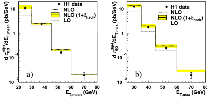
Fig. 2a,b. Differential ep cross sections for dijet production ( Q^2 < 1\text{GeV}^2 ) as a function of a E_{T,mean} , the mean and b E_{T,max} , the maximum E_T of the two highest E_T jets. The LO predictions using CTEQ5M pdfs for the proton and GRV-HO pdfs for the photon are shown as a dotted line . NLO predictions with the same pdfs are shown as a dashed line . The full line shows the NLO predictions, including hadronization corrections and the grey band indicates the renormalization and factorization scale uncertainties of the NLO prediction
