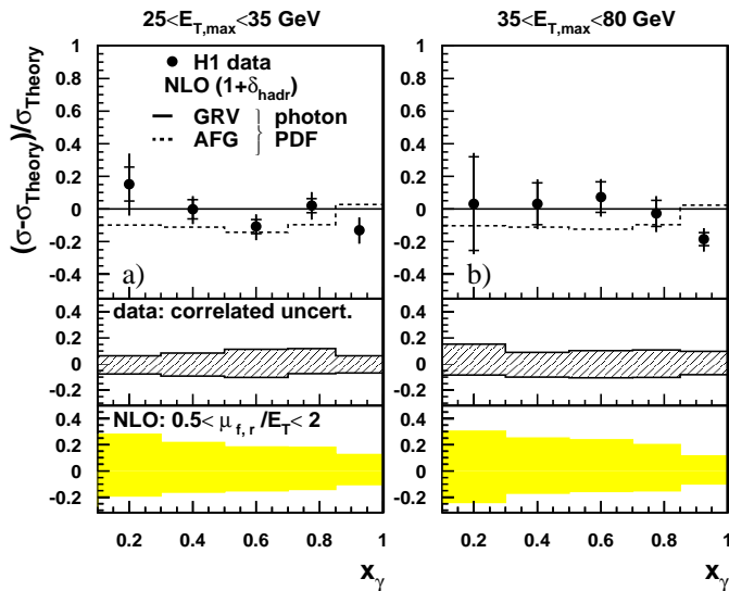
Fig. 7a,b. The x_\gamma dependence of the relative difference of the measured dijet cross sections ( Q^2 < 1\text{GeV}^2 ) from the NLO prediction, with hadronization corrections applied using CTEQ5M pdfs for the proton and GRV-HO pdfs for the photon (here \sigma_{Theory} ). The symbol \sigma stands for d\sigma/dx_\gamma . Shown is the relative difference of the data (points) and the NLO predictions using the AFG-HO pdf (dashed line) with hadronization corrections applied. a and b show the relative difference for the lower E_{T,max} and higher E_{T,max} regions respectively. The inner error bars denote the statistical error, the outer error bars denote all statistical and uncorrelated systematic errors of the data added in quadrature. The correlated systematic errors are shown in the middle plots as a shaded band. The grey band (lower plots) shows the renormalization and factorization scale uncertainties of this NLO prediction
