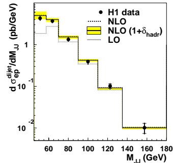
Fig. 1. Differential ep cross section for dijet production ( Q^2 < 1\text{GeV}^2 ) as a function of the invariant dijet mass M_{JJ} of the two highest E_T jets. Here, as well as in the following figures unless explicitly stated otherwise, the inner error bars denote the statistical error, the outer error bars the total uncertainties of the data. The LO predictions using CTEQ5M pdfs for the proton and GRV-HO pdfs for the photon are shown as a dotted line . NLO predictions with the same pdfs are shown as a dashed line . The full line shows the NLO predictions, including hadronization corrections and the grey band indicates the renormalization and factorization scale uncertainties of the NLO prediction
